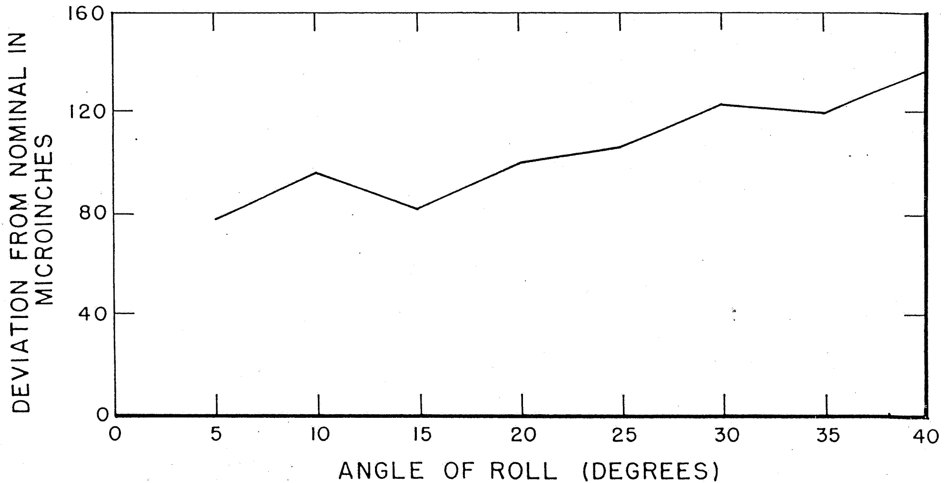
PLOT OF INVOLUTE PROFILE ERRORS FROM NOMINAL WITH DATA FROM FIGURE 17
